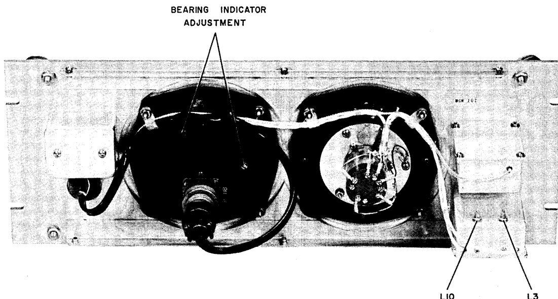
Figure 5-3. 477U-2 ADF Antenna Simulator Adjustments
