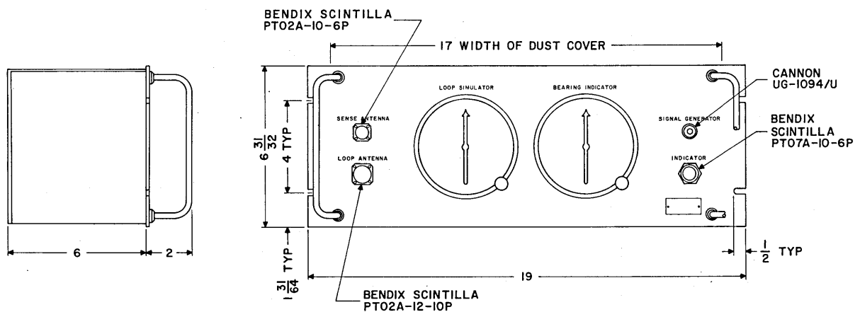
Figure 2-1. 477U-2 ADF Antenna Simulator, Outline and Mounting Dimensions
