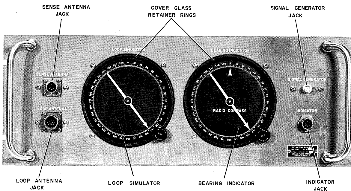
Figure 3-1. 477U-2 ADF Antenna Simulator, Front Panel
