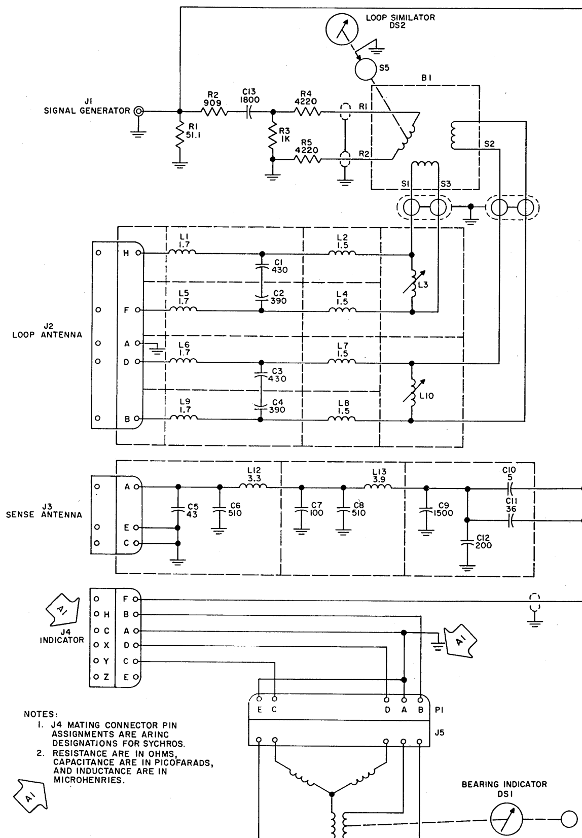
Figure 7-1. 477U-2 ADF Antenna Simulator, Schematic Diagram
