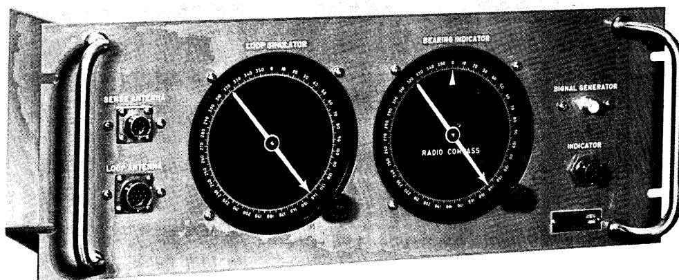
477U-2 ADF ANTENNA SIMULATOR
