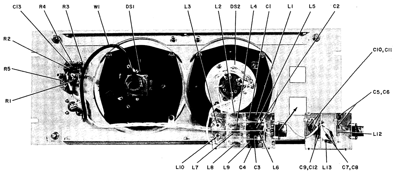
Figure 6-1. 477U-2 ADF Antenna Simulator, Rear View, Cover Removed
