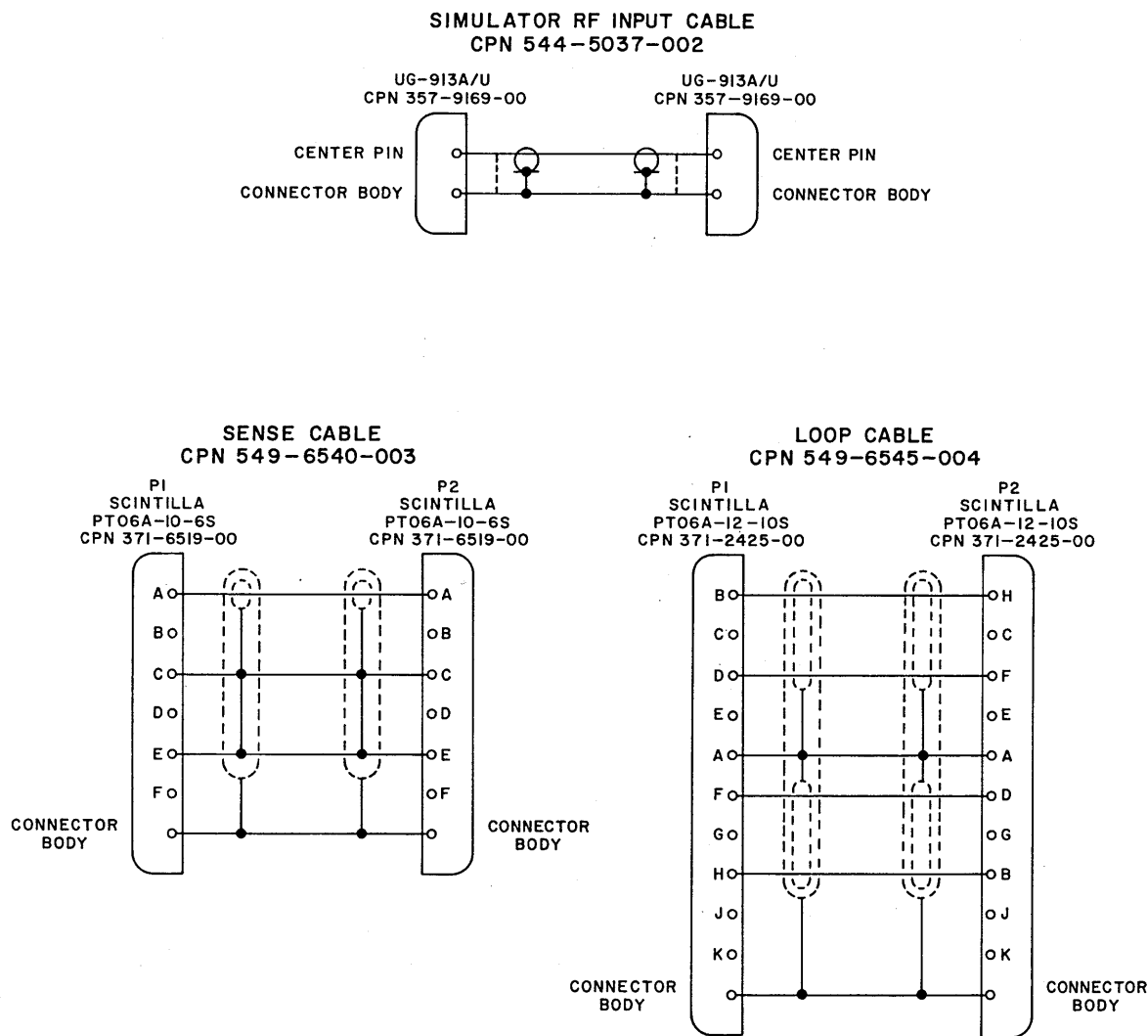
Figure 7-2. Simulator R-F Input Cable, Sense Cable, and Loop Cable, Schematic Diagram
