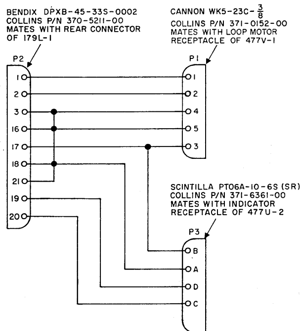
Figure 3-2. 179L-1 Interconnection Test Cable, Schematic Diagram
